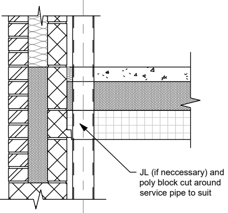
JF154 - Service Pipe Tight to Wall
