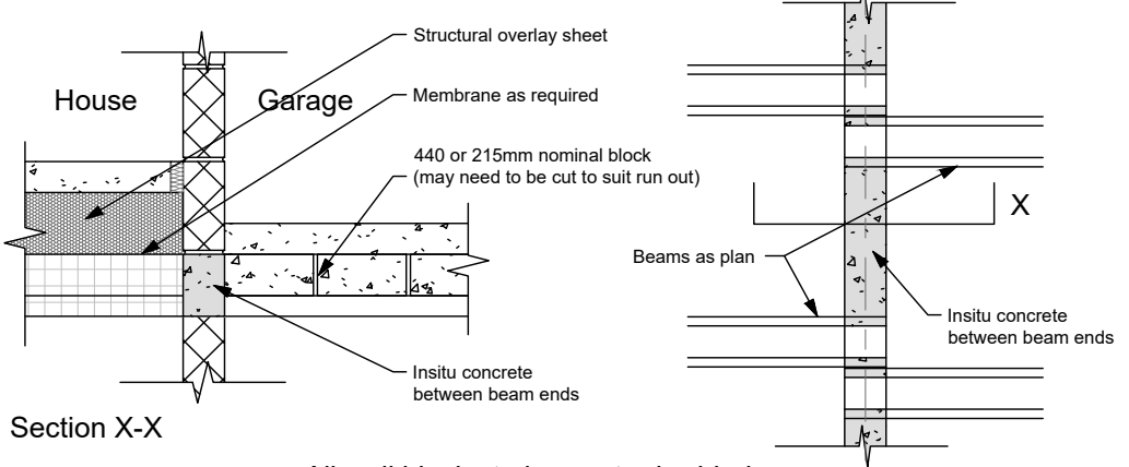
JF153 - Staggered Bearing Loadbearing Wall
